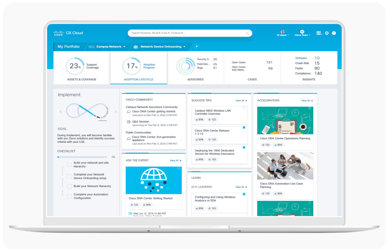
Figure 2. CX Cloud
