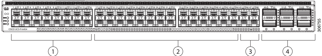
Figure 5 6454 54-port Fabric Interconnect Chassis Overall Rear View
